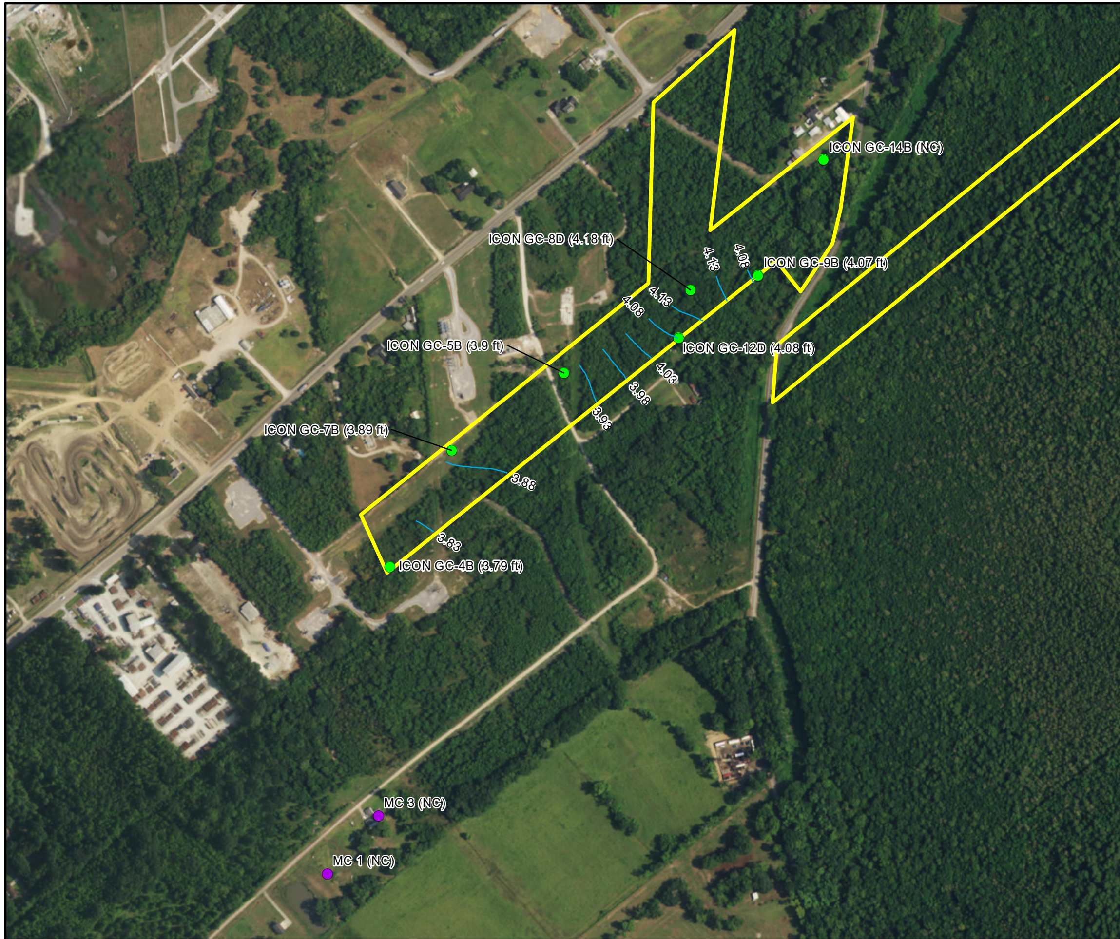
FIGURE 24 DENSITY ADJUSTED GROUNDWATER ELEVATIONS FOR AUGUST 22, 2016 -25 to -60 ft Elevation Between 45 ft and 78 ft bgs (approx)
