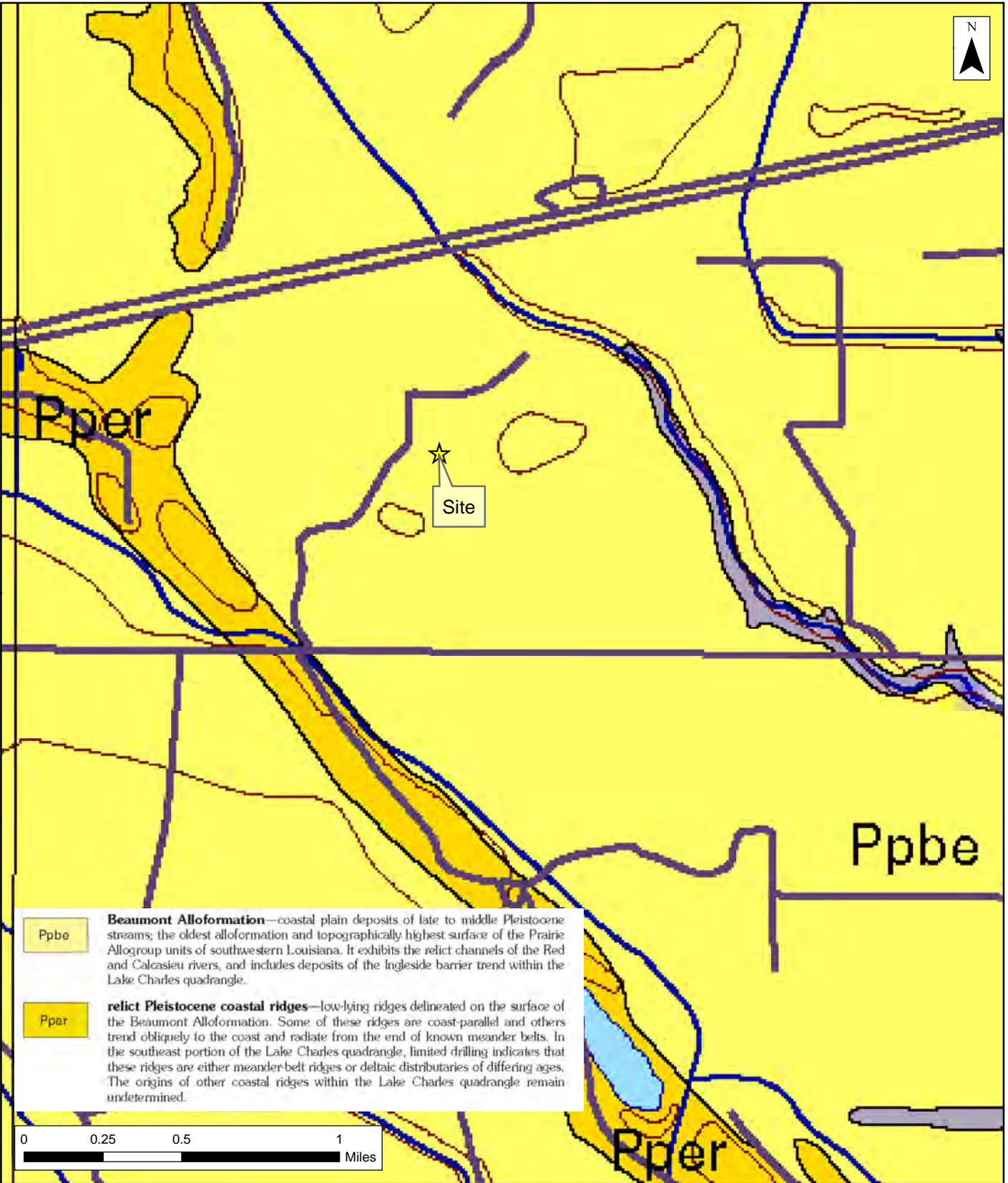
Figure 9 Surface Geology H. C. Drew Estate vs Neumin Production Company North Choupique Field Calcasieu Parish, Louisiana
