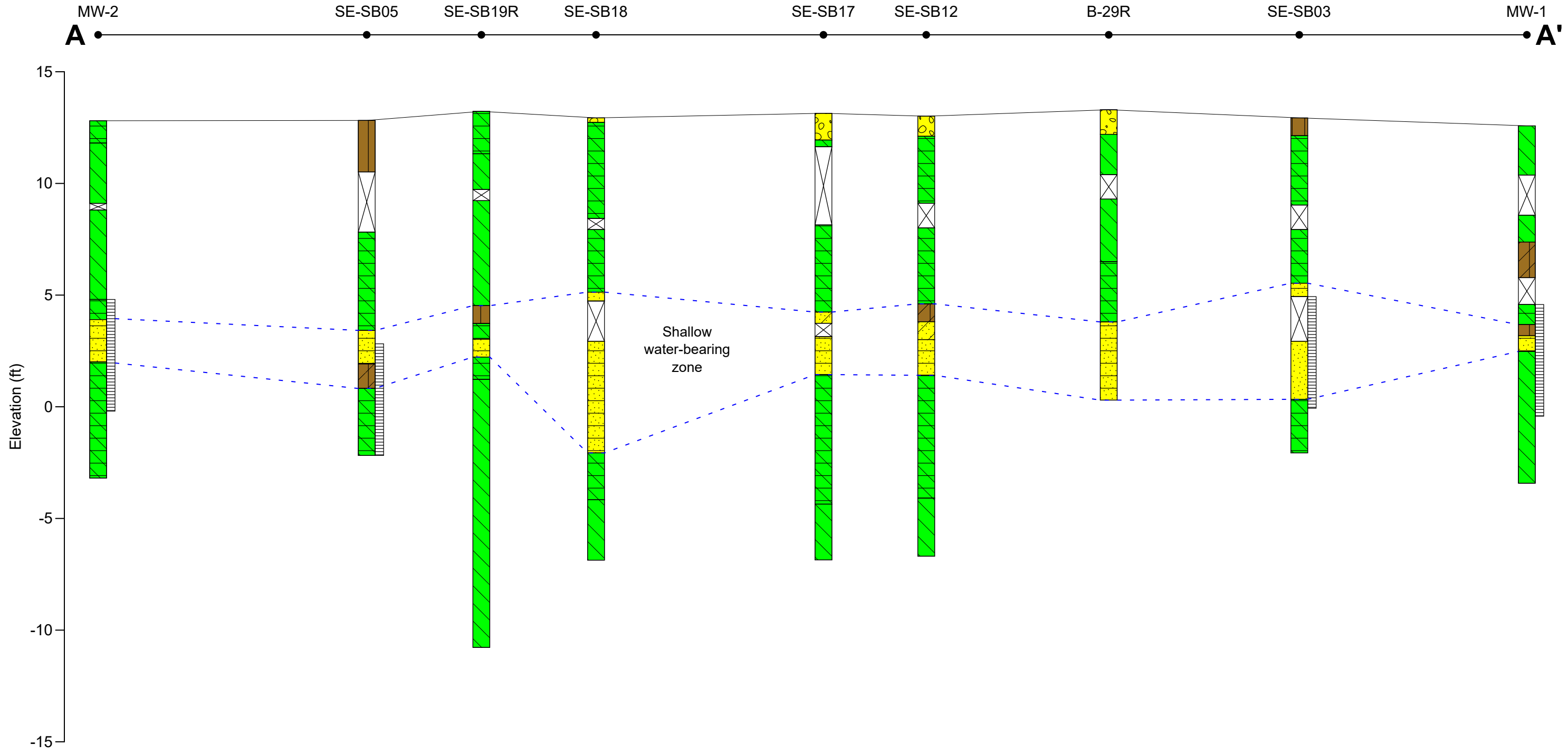
Figure 11 Cross Section A to A' H. C. Drew Estate vs Neumin Production Company North Choupique Field Calcasieu Parish, Louisiana
