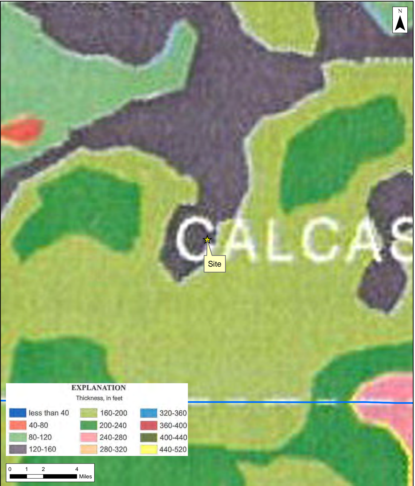
Figure 13 Thickness of Chicot Confining Unit H. C. Drew Estate vs Neumin Production Company North Chouiquie Field Calcasieu Parish, Louisiana
