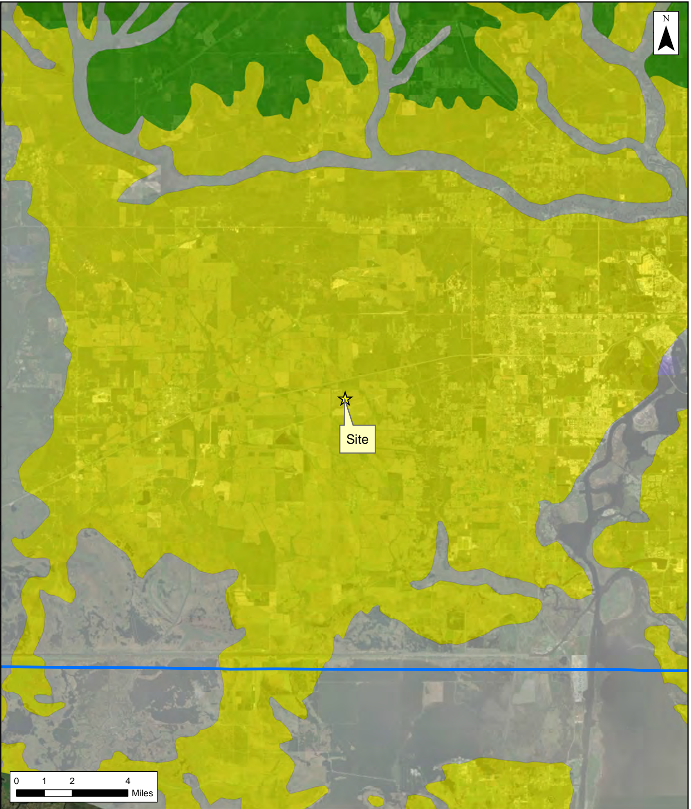
Figure 15 Louisiana Aquifer Recharge Potential H. C. Drew Estate vs Neumin Production Company North Chouiquie Field Calcasieu Parish, Louisiana
