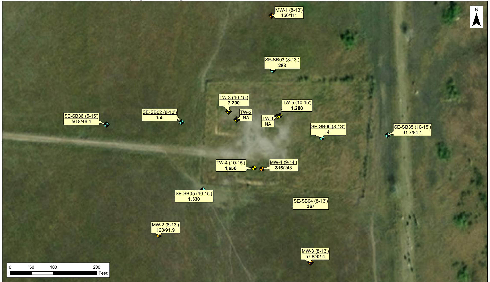
Figure 42A Chloride in Groundwater - Zoom H. C. Drew Estate vs Neumin Production Company North Choupique Field Calcasieu Parish, Louisiana
