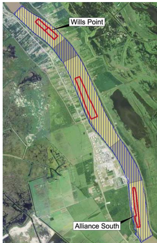
Figure 1. Multibeam (Blue Hatched) and the two Magnetometer Survey Areas.
