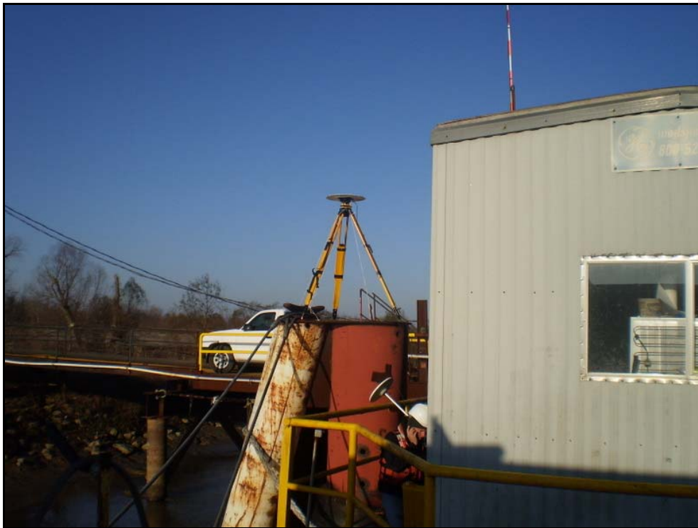
Figure 2. RTK GPS Base Station Deployed at "AEP WASH."
